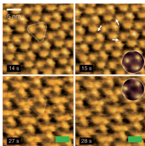
Figure 1. HS-AFM images of the D96N bR mutant at the cytoplasmic surface. 1 frames -1 , 200×200 pixels. The membranes were adsorbed onto a mica surface in 10 mM phosphate (pH 8) and 300 mM KCl. A bR trimer is highlighted by the white triangles. The white arrows indicate the direction of the conformational change in bR (15 s). The green bars indicate application of 532 nm green light (27 and 28 s). The insets in the images at 15 and 28 s are averaged images of a bR trimer captured in the dark and under green light, respectively.
